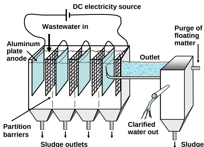
Fig. 12. Schematic illustration of an electrocoagulation system in which an aluminum electrode serves as the anode, releasing soluble ionic species of aluminum (redrawn based on a system studied by Pérez-Sicairos et al. (2011))
